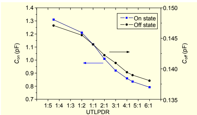
Fig. 3. Calculated C_{on} and C_{off} versus UTLPDR.
