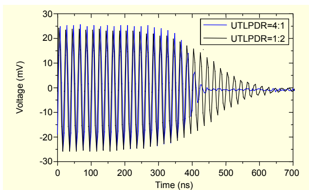
Fig. 5. Measured falling times for two types of SPDT MMIC switches.
