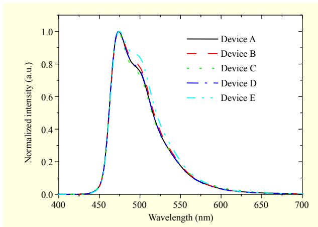
Fig. 3. Normalized EL spectra of Devices A through E at driving current of 10 mA/cm 2 .
