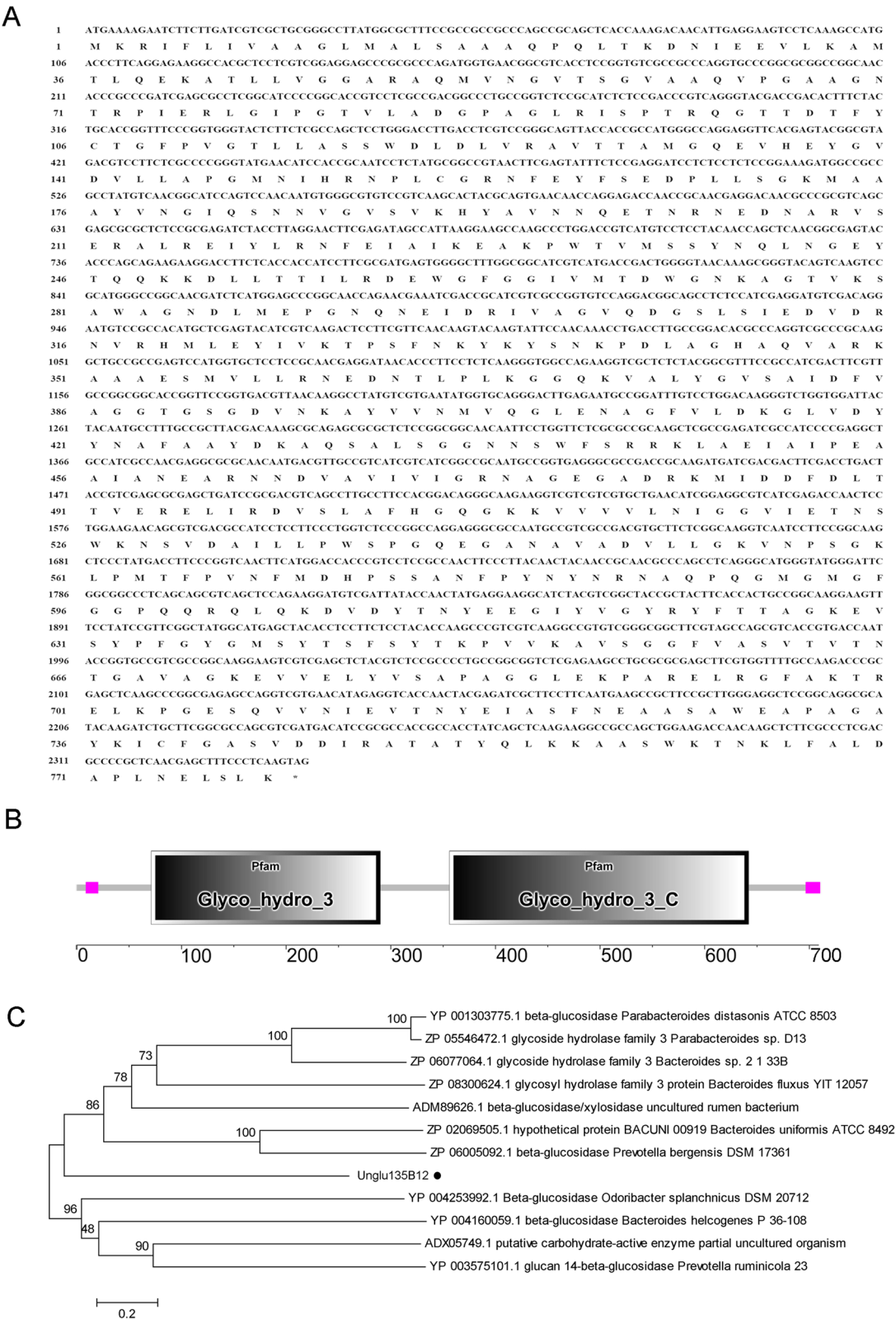
Figure 2 Characterization of amino acid sequence of Unglu135B12. A amino acid sequence of Unglu135B12. B Predicted modular architecture of Unglu135B12. C Phylogenetic relationship of Unglu135B12 with related proteins. The scale bar corresponds to a genetic distance of 0.2 substitutions.
