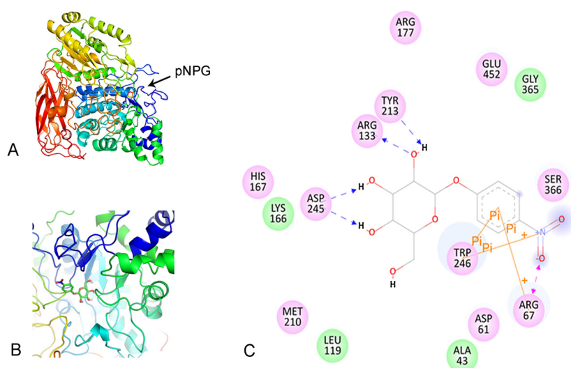
Figure 5 Structural models of \beta -glucosidases Unglu135B12 characterised in the present work and its substrate docking. A. The pNPG-binding model of Unglu135B12 derived from Thermotoga neapolitana \beta -glucosidase 3B (PDB ID 2X40). The three protein domains: \alpha/\beta barrel, \alpha/\beta sandwich and fibronectin-like, were coloured cyan, blue and red, respectively. B. Closeup of the catalytic centre. C. The key residues in the catalytic pocket around pNPG.
