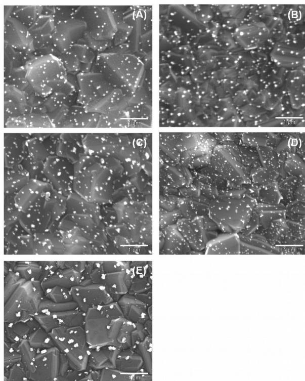
Figure 3. SEM images of microcrystalline diamond thin-film electrodes decorated with Pt metal particles using pulsed galvanostatic deposition at current densities from 0.05 to 1.50 \text{mA/cm}^2 .
