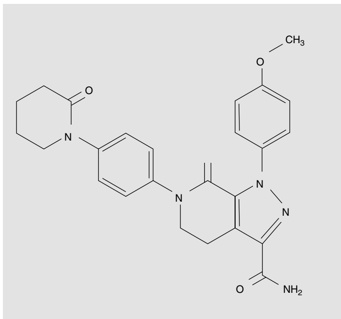
FIGURE 3.3 Apixaban
