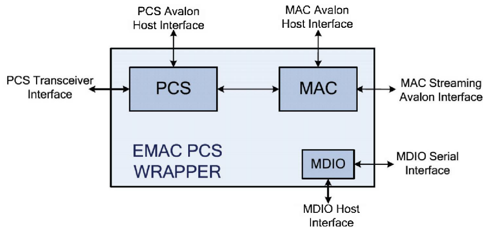
Fig. 2 – 40 G MAC PCS Wrapper Architecture
